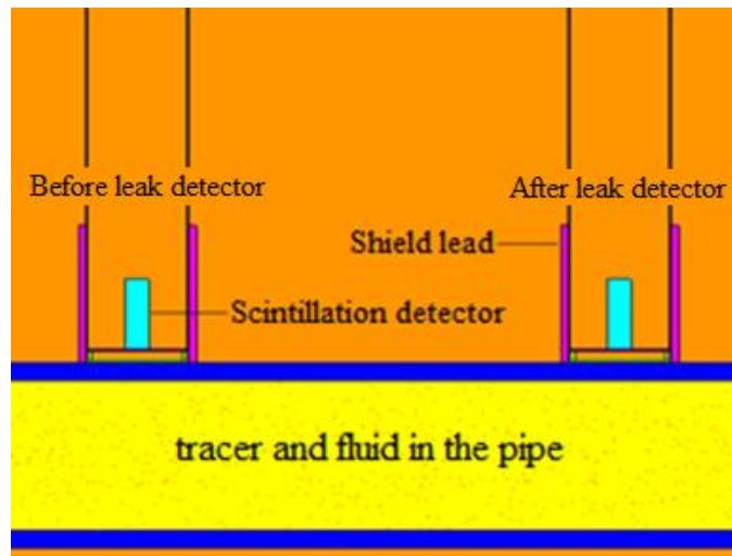
Figure 2. Schematic view of leakage measurement configuration in the pipe.
