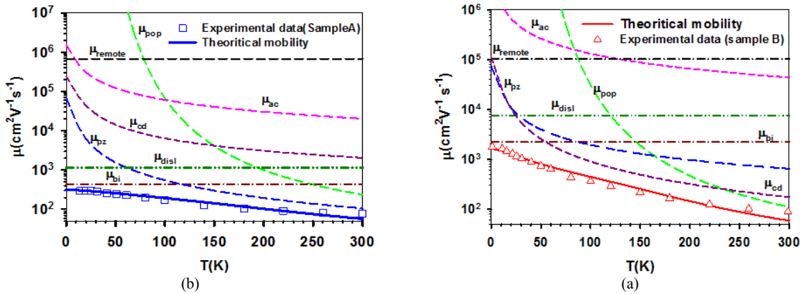
Figure 5. Experimental and calculated temperature dependence of electron mobility curves for (a) \text{Zn}_{0.82}\text{Mg}_{0.18}\text{O}/\text{ZnO} and (b) \text{Zn}_{0.8}\text{Mg}_{0.2}\text{O}/\text{ZnO}/\text{graded-Zn}_{0.85}\text{Mg}_{0.15}\text{O} .
