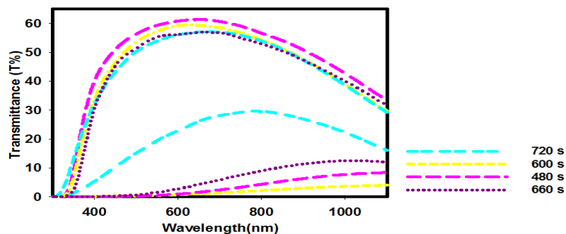
Figure 2. (color online) Optical transmittance spectra of the \text{WO}_3 thin layer with different deposition times in the colored and bleached states within the 300 \leq \lambda \leq 1100 nm range.
