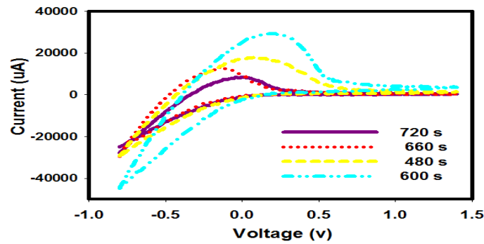
Figure 3. (color online) Cyclic voltamogram for WO 3 thin layers with different deposition times.
