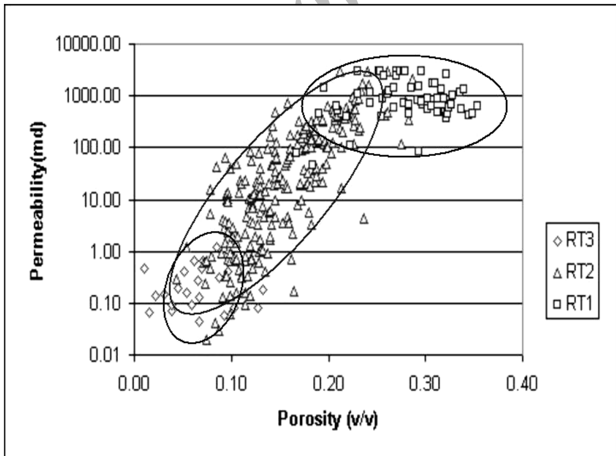
Fig. 1. Permeability versus porosity, siliciclastic reservoir rock types.
