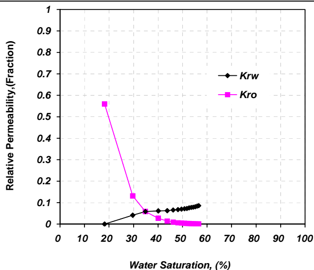
Fig. 1- Typical relative permeability curve for sample.
