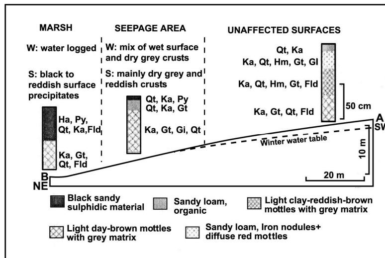
Fig. 2 A soil toposéquence across the acid saline seep affected landform showing the main surface and subsurface soil morphological features. W–winter (wet) season, S–summer (dry). Mineralogy of individual soil horizon morphologies only: Qt–quartz, Ka–kaolinite, Hm–hematite, Gt–goethite, Gi–Gibbsite, Ha–halite, Py–pyrite, Fld–feldspar.
