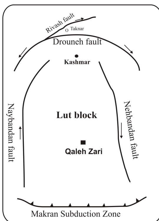
Figure 2 Map showing the location of Qaleh Zari mine in central Lut region.
