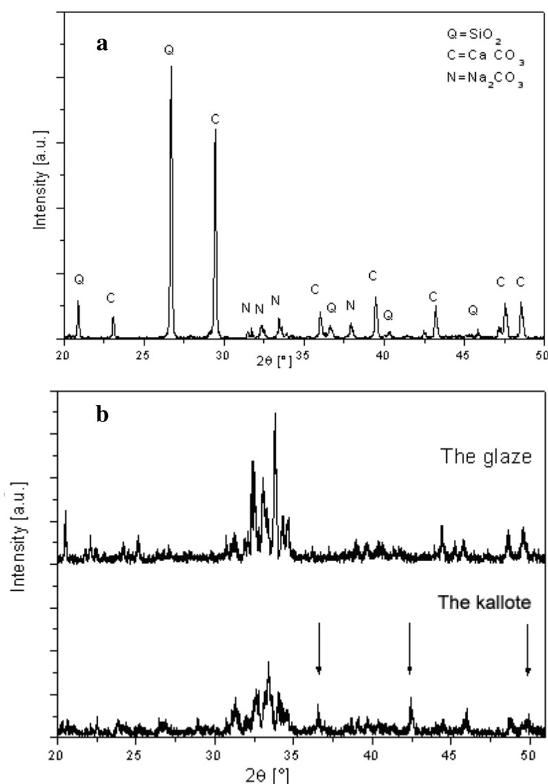
Fig. 3. A) X-Ray diffraction pattern of the raw materials for the coatings powders. Q=Quartz ( SiO_2 ), C=Calcite ( CaCO_3 ), N=Sodium Carbonate ( Na_2CO_3 ). B) X-ray diffraction pattern of the porous part around the glazes (Kallotte) and of the surfaces of glazes. The arrows indicate the presence of the CoO-pigment.
