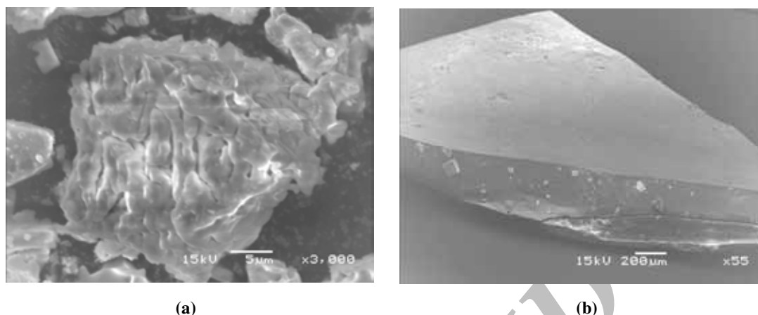
Fig. 4. SEM image showing the microstructure and morphology of: (a) porous Kallote and (b) The glazed side.
