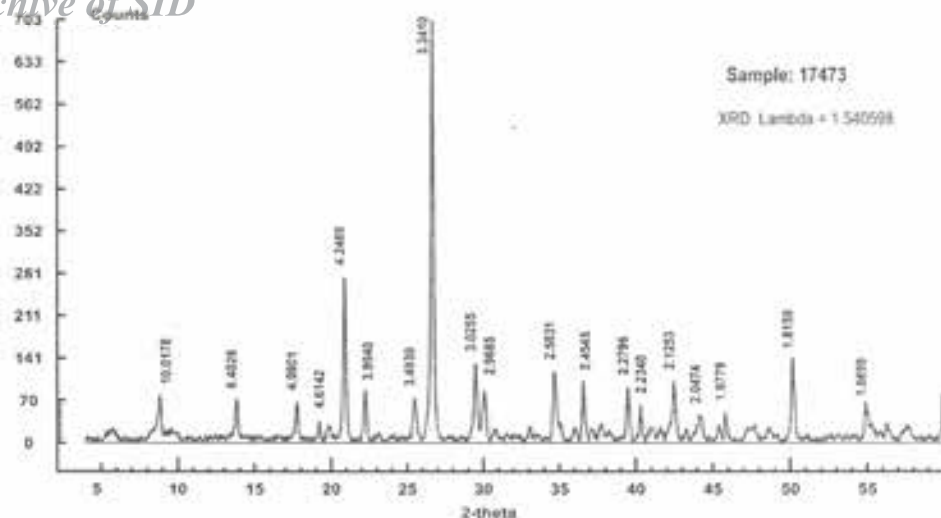
Figure 2c X-ray diffraction graph of Hired tourmaline.
