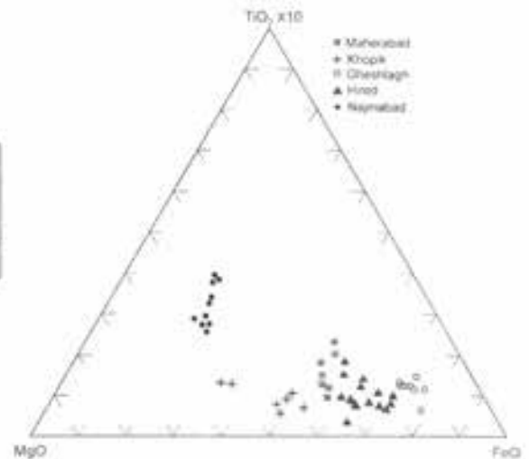
Figure 6 Ternary MgO-FeO-TiO_2 diagram shows the composition of tourmaline from the five study areas.
