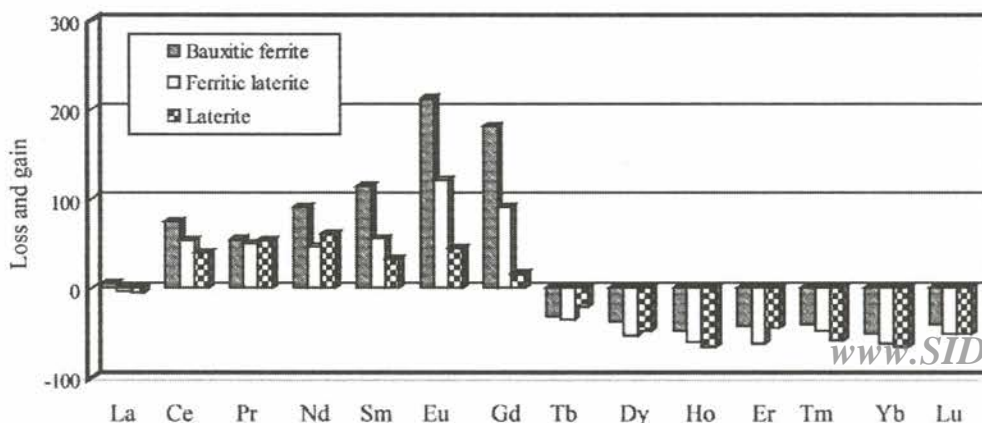
Fig.13 Mass changes for rare earth elements (REE) during the formation of various lateritic types at studied area.
