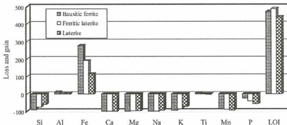
Fig.11 Mass changes for major, and minor elements as well as LOI during the formation of various lateritic types at studied area.
