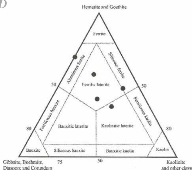
Fig.6 Position of data points of the lateritic ores at studied area on a trivariate plot of Fe-bearing minerals (hematite and goethite), clays (kaolinite and other clays), and free aluminum (gibbsite, boehmite, diaspore, and corundum) [7].
