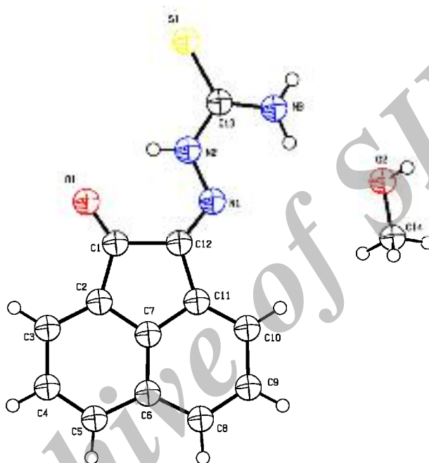
Fig. 1. ORTEP diagram of 1 . Thermal ellipsoids are at 50% probability level.
