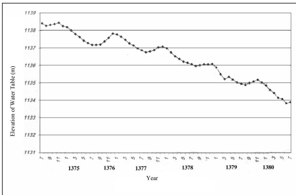
Fig.1. Neishabour Plain Hydrograph (Elevation of Water Table)
