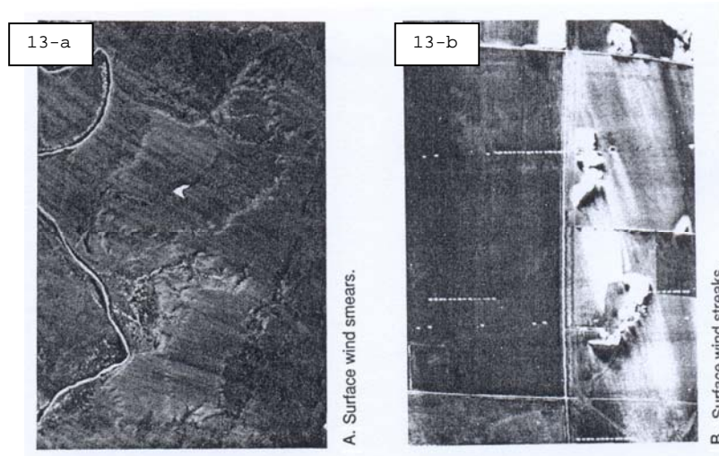
Fig. 13. IRS images affected by wind
