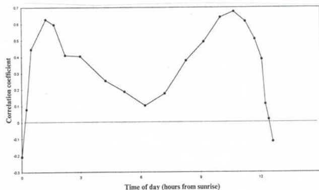
Fig. 16. Correlation between reflective & thermal images on desert surface
