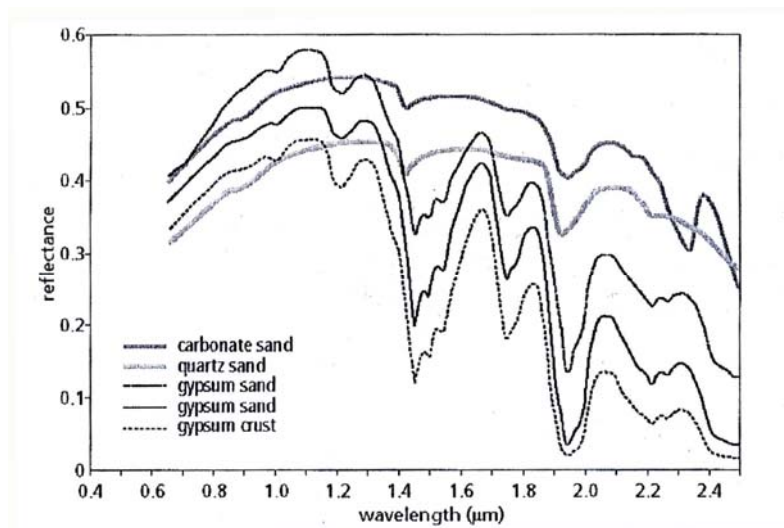
Fig. 7-b. Hypespectral Spectral curve with high resolution for carbonate sand, quartz sand, gypsum sand and gypsum crust
