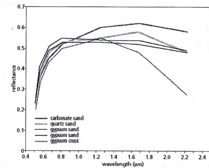
Fig. 7-a. Multispectral Spectral curve with low resolution carbonate sand, quartz sand, gypsum sand and gypsum crust
