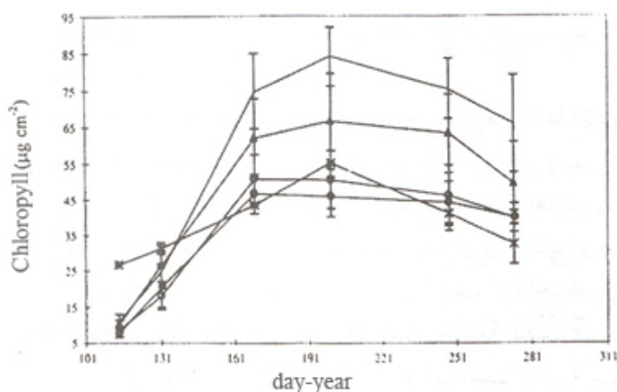
Fig. 5. Chlorophyll concentration measured in leaves of some plants between April and September: sun-exposed leaves of oak (—○—), shaded leaves of oak (—△—), sun-exposed leaves of beech (---○---), shaded leaves of beech (---□---)
