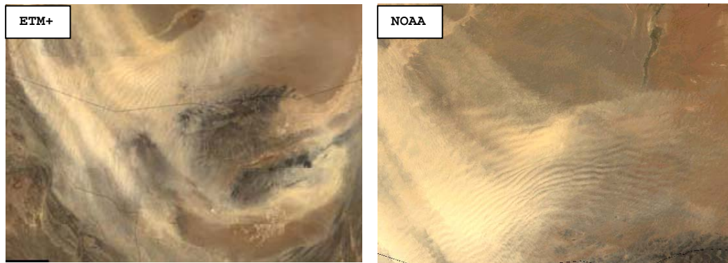
Fig. 14. Wind effect on formation of sand storms in Sistan region (AVHRR & ETM+ images)
