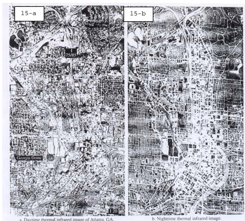
Fig. 15. Thermal IR (band 13, 9.6-10.2 \mu\text{m} ), Atlanta city: (a) Day Thermal IR, (b) Night Thermal IR (Jensen, 2000)
