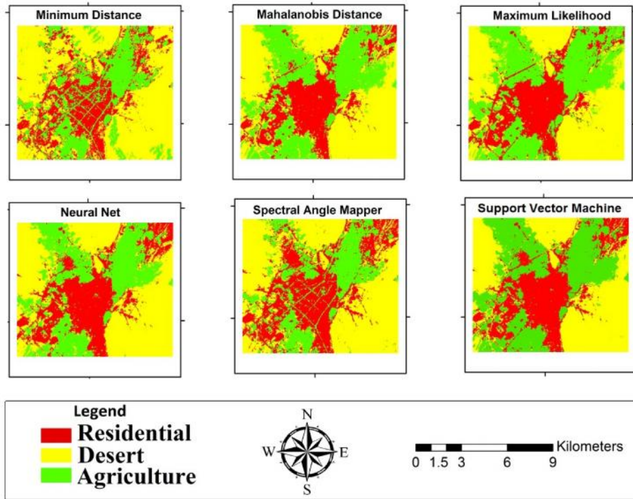
Fig. 2. Land use maps with 6 classification algorithms for Shahreza
