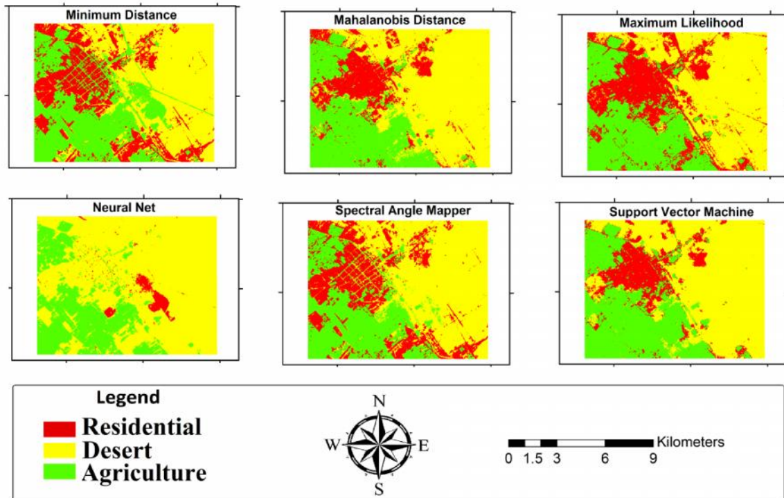
Fig. 4. Land use maps with six classification algorithms for Zarand
