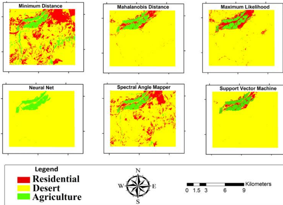
Fig. 3. Land use maps with six (6) classification algorithms for Taft
