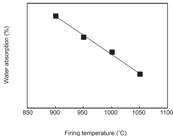
Figure 8. Effect of maximum firing temperature on water absorption of lightweight brick with 1.5 wt.% polystyrene foam additive.
