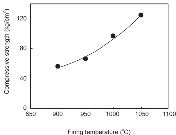
Figure 7. Changes in compressive strength of lightweight brick made by 1.5 wt% polystyrene foam vs. maximum firing temperature.
