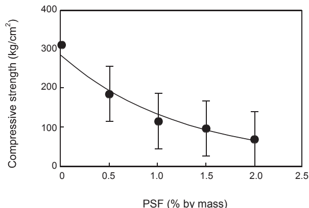
Figure 5. Compressive strength of brick samples vs. polystyrene foam content.
