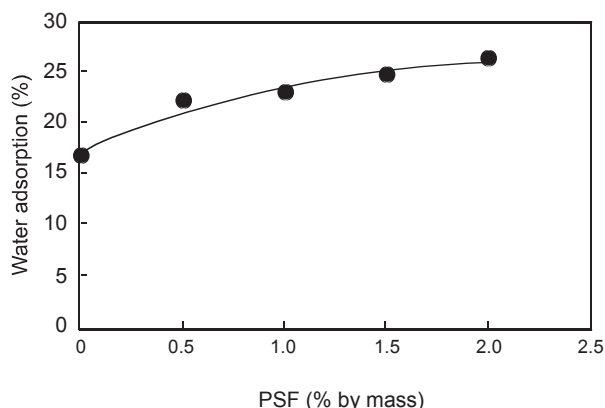
Figure 4. Effect of polystyrene foam content on water adsorption of brick samples.
