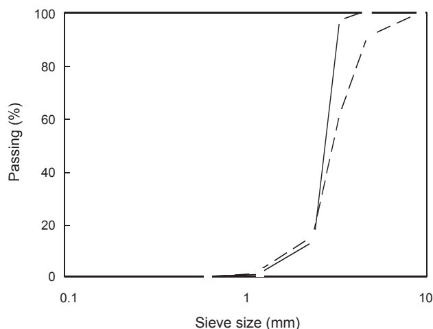
Figure 2. Particle size distribution of virgin and recycled polystyrene foam. —□— recycled PSF; —○— virgin PSF.
