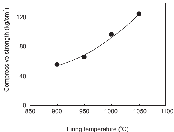
Figure 7. Changes in compressive strength of lightweight brick made by 1.5 wt% polystyrene foam vs. maximum firing temperature.
