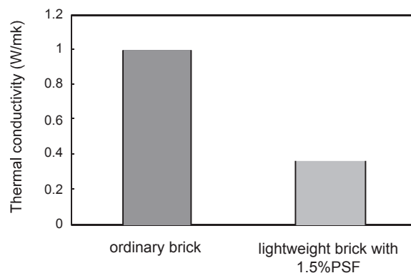
Figure 9. Comparison of thermal conductivity of lightweight bricks with polystyrene foam (1.5 wt. %) and ordinary bricks.
