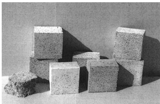
Figure 1. Lightweight brick samples made with PS foam pore forming additive.
