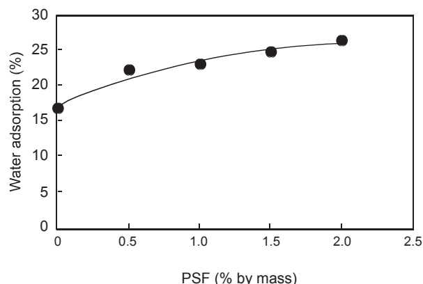
Figure 4. Effect of polystyrene foam content on water absorption of brick samples.
