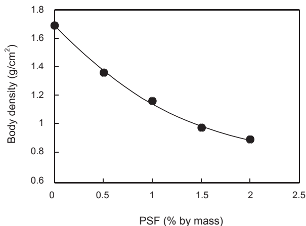
Figure 3. Body density of the brick samples vs. polystyrene foam content.
