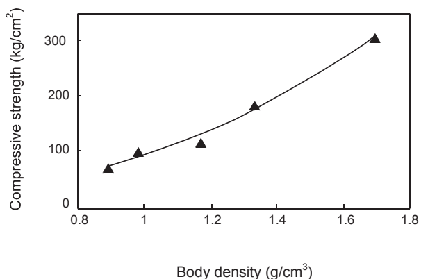
Figure 6. Relationship between the compressive strength and body density in bricks made with different PSF contents.
