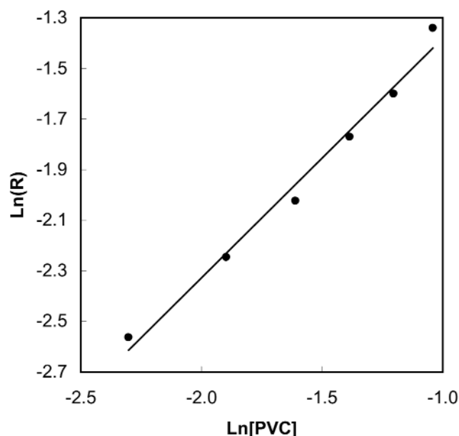
Figure 7. \text{Ln}(R) vs. \text{Ln}[\text{PVC}] in absence of stabilizer at 180^\circ\text{C} .
