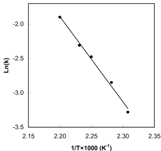
Figure 8. \text{Ln}(k) vs. 1/T for degraded PVC.
