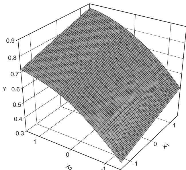
Figure 1. Dependence of DS_{ph} ( Y ) on molar ratios of catalyst /CA ( x_1 ) and phthalic anhydride/CA ( x_2 ) for the phthaloylation of CA in acetic acid medium.
