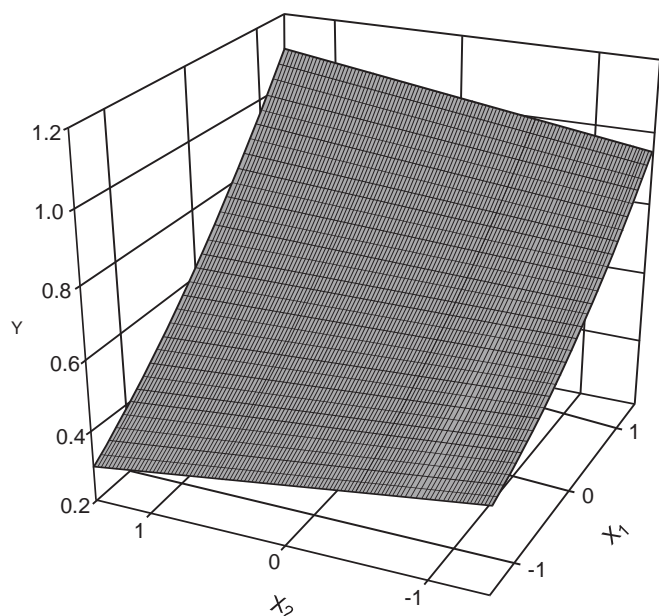
Figure 2. Dependence of DS_{ph} ( Y ) on molar ratios catalyst / CA ( x_1 ) and phthalic anhydride/CA ( x_2 ) for the phthaloylation of CA in acetone medium.
