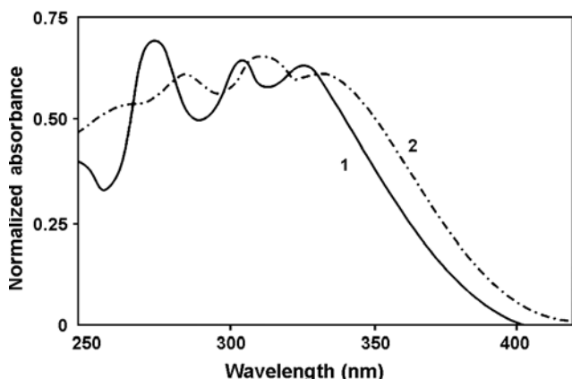
Figure 3. Absorption spectra of: (1) 2-PIMP and (2) O-2-PIMP.
