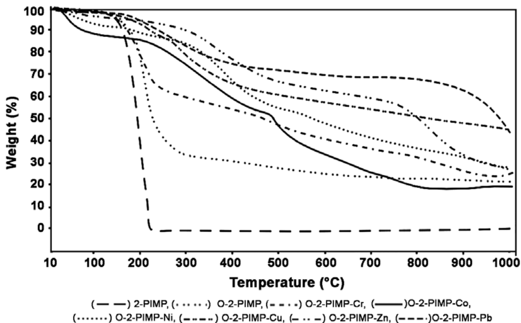
Figure 6. TGA Curves of 2-PIMP, O-2-PIMP, and O-2-PIMP-metal complexes.
