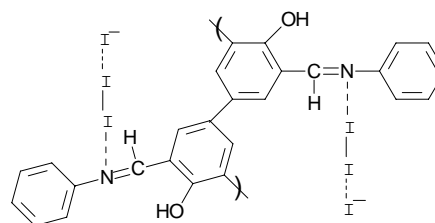
Scheme IV. Coordination of iodine during O-2-PIMP doping.
