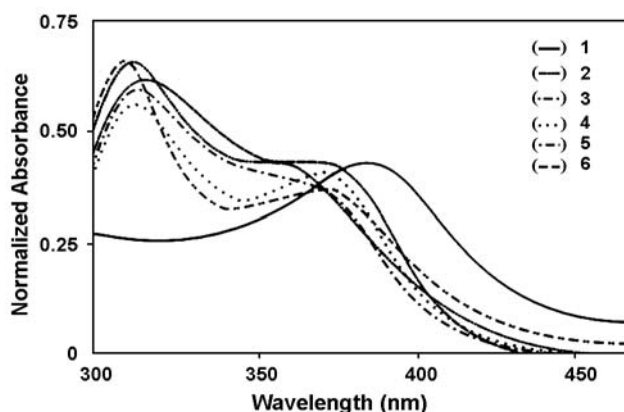
Figure 4. Absorption spectra of oligomer-metal complexes (1= Cu 2+ , 2= Ni 2+ , 3= Co 2+ , 4= Cr 3+ , 5= Pb 2+ and 6=Zn 2+ ).
