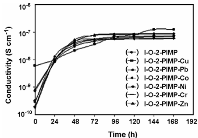
Figure 5. Electrical conductivity of I 2 -doped O-2-PIMP and its metal complexes vs. doping time at 25°C.
