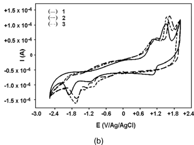
Figure 2. Cyclic voltammograms of 1 mM oligomer metal complexes of: (a) 1= Cu +2 ; 2= Ni +2 ; 3=Co +2 and (b) 1= Cr +3 ; 2= Pb +2 ; 3=Zn +2 in DMSO at a sweep rate of 250 mV s -1 .
