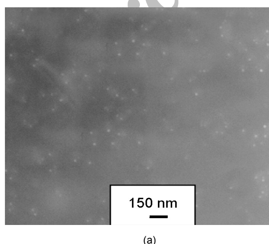
Figure 4. TEM Images of microemulsions at different amounts of catalyst: (a) 1.0 wt% and (b) 5.0 wt%.
