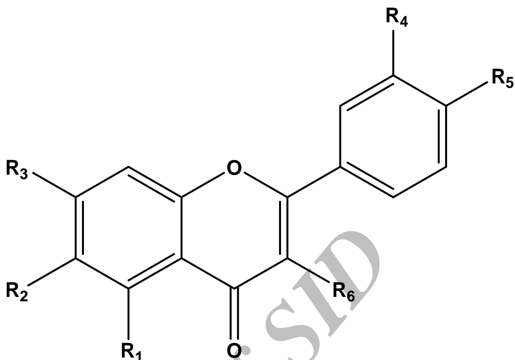
Salvigenin: R_1 = \text{OH} , R_2 = \text{OMe} , R_3 = \text{OMe} , R_4 = \text{H} , R_5 = \text{OMe} , R_6 = \text{H} Santoflavone: R_1 = \text{H} , R_2 = \text{OMe} , R_3 = \text{OH} , R_4 = \text{OMe} , R_5 = \text{OMe} , R_6 = \text{OMe}
