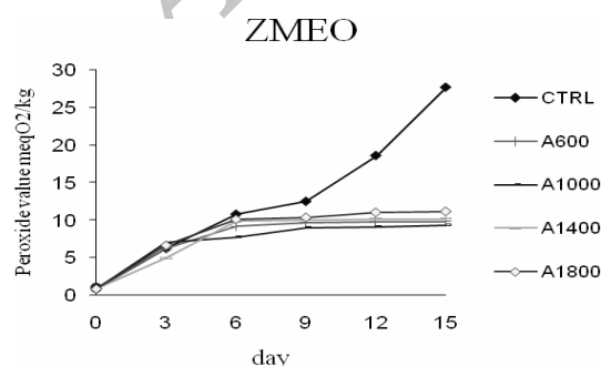
Figure 6- Changes of PV of linseed oil containing ZMEO and BPEO as natural antioxidant after heating at 60°C for 15 days
