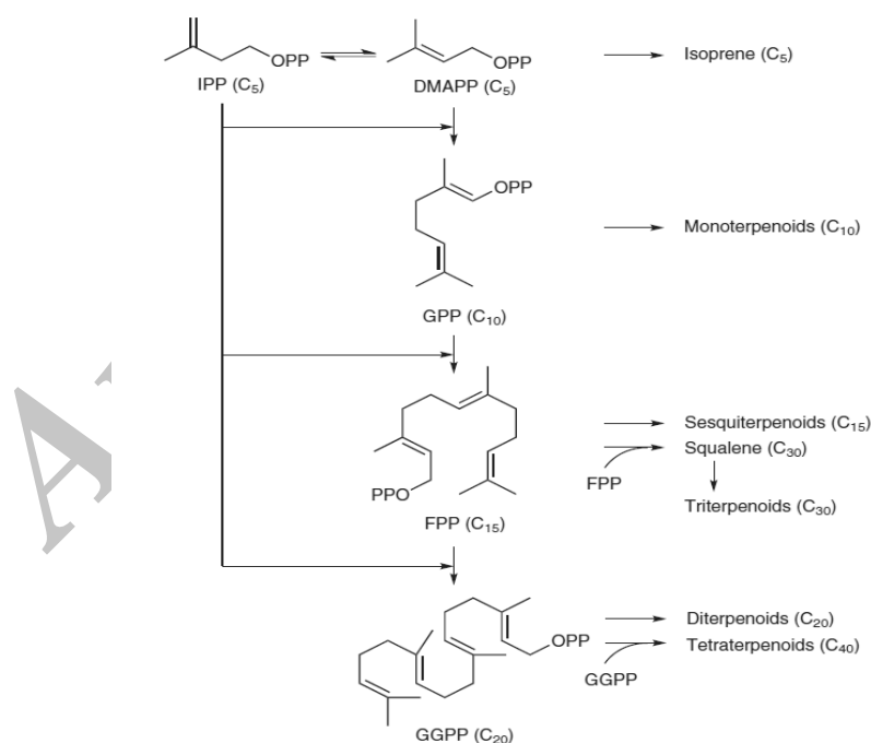
Figure 2- Overview of terpenoid biosynthesis and the generation of terpenoid starting blocks. Isopentenyl diphosphate (IPP) and dimethylallyl diphosphate (DMAPP) condense to form higher order terpenoid precursors, including the monoterpenoid precursor geranyl diphosphate (GPP), the sesquiterpenoid precursor farnesyl diphosphate (FPP) and the diterpenoid precursor geranylgeranyl diphosphate (GGPP). Two molecules of FPP condense to form the triterpenoid precursor squalene, and two molecules of GGPP condense to form higher order tetraterpenoids [10]
