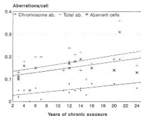
Fig. 1: Relations between deferent types of aberration and the years of cronic exposure
