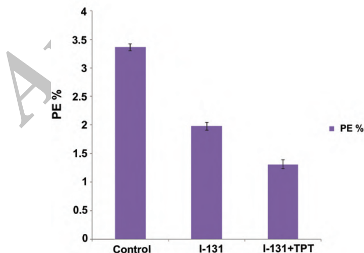
Fig.7: Plating efficiency (PE) for glioblastoma (GBM) cell line in control, iodine- 131 (I-131)+topotecan (TPT) and I-131 groups. Data are presented as mean \pm standard error of the mean (SEM).
