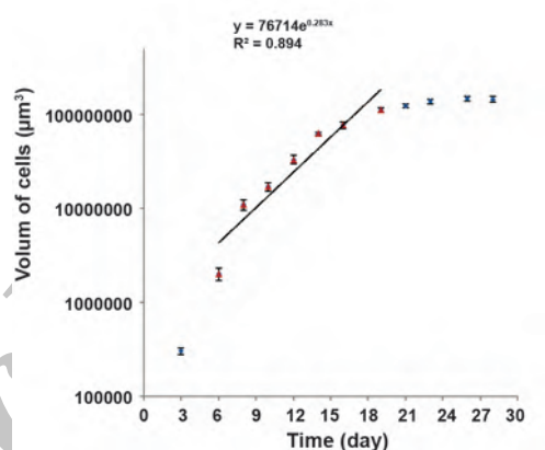
Fig.2: Growth curve of U87MG cell line in spheroid Cultures. An average of nine counts was used to define each point. Mean \pm SEM of three experiments is shown on the curve.
