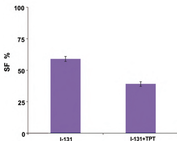
Fig.8: Fraction of cells that survived for the glioblastoma (GBM) cell line in the iodine-131 (I-131)+topotecan (TPT) and I-131 groups. Data are presented as mean \pm SEM. SEM; Standard error of the mean and SF; Survival factor.
