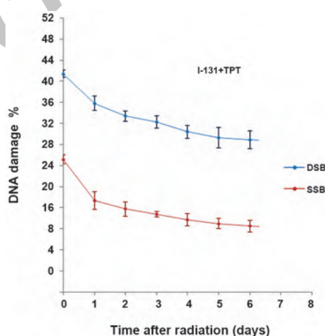
Fig.6: Distribution of the average percentage of single-strand breaks (SSB) and double-strand breaks (DSB) of glioblastoma (GBM) cells in groups irradiated with 2Gy of beta iodine (I-131) and treated with topotecan (TPT) after 7 days of radiation and treatment. Data are presented as mean \pm standard error of the mean (SEM).
