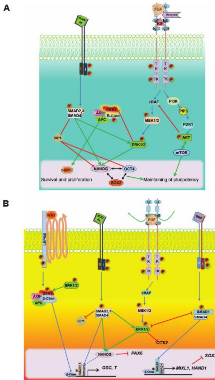
Fig.1: Molecular interplay of FGF and NODAL signaling in maintenance of pluripotency in hPSCs and mesendodermal differentiation. A. Self-renewal of hPSCs depend on activation of both fibroblast growth factor (FGF) and activin/nodal signals. Activin/Nodal signals bind to type II receptors. Heterodimerization of receptors and their phosphorylation results in activation of R-Smads (SMAD2/3) and their binding to the co-SMAD (SMAD4). Internalization of the SMAD protein complex to the nucleus activates expression of NANOG directly. Indirectly, this could sustain the core pluripotency network and expressions of OCT4 and SOX2. SMAD proteins also inhibit expression of the SMAD interacting protein (SIP) which has a negative effect on OCT4 and NANOG expression, and could enhance neuroectodermal differentiation. FGF activation, by binding of their ligands [FGF, insulin-like growth factor (IGF) and heregulin] to tyrosine kinase receptors, results in phosphorylation and activation of phosphatidylinositol 3-kinase (PI3K) and cRAF. Activation of PI3K in turn activates AKT, which is involved in mediating inhibition of apoptosis and stimulation of cell proliferation, specifically via mTOR signaling in human pluripotent stem cells (hPSCs). Activation of cRAF activates mitogen-activated protein kinase MEK/ERK signaling that controls cellular processes such as survival and differentiation, and can maintain NANOG expression. A moderate signal of internal glycogen synthase kinase-3 (Gsk3) in hPSCs is needed for cell proliferation via c-Myc expression and B. Combined signals of mesendodermal specification. Activation of p-SMAD2/3 downstream of activin/nodal external signals reinforces the expression of NANOG and primitive streak specific genes (GSC and T). The high expression level of the ERK signaling, downstream of FGF, helps to stabilize the expression of β-ctnn and the mesendodermal genes. Phosphorylation of SMAD1 and its dimerization with SMAD4 occurs as a result of BMP binding to its receptors which enhance the expression of the posterior mesoderm and extra-embryonic mesodermal genes (Hand1 and Mixl1). Expressions of neural specific genes (SIP1, PAX6, OTX2 and SOX2) that are inhibited by mesodermal signals are depicted by red lines.
