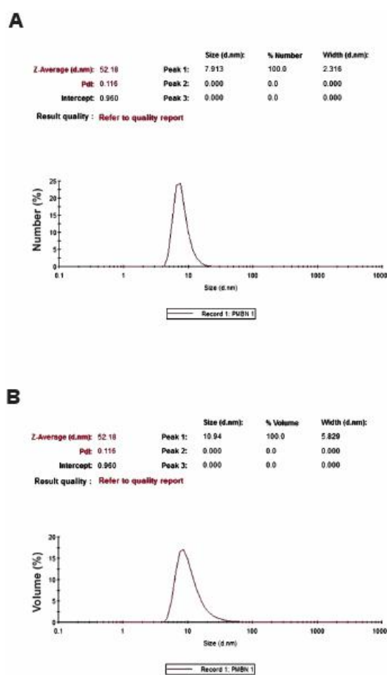
Fig.4: Size of polymer was analyzed by dynamic light scattering (DLS) to figured out it was had nano structure or not. A. Measurement based on number index that showed a mean diameter of 52.18 nm, B. Measurement based on volume index that indicated a mean diameter of 52.18 nm, and C. Measurement based on intensity index that determined the polymer size at 52.18 nm. The poly dispersity index (PDI) of PMBN was 0.116.
