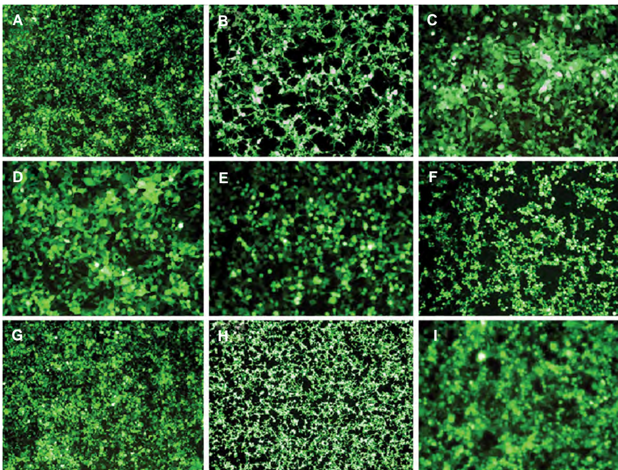
Fig.1: Transfection efficiency of lentiviral anti- ADK miR-shRNAs vectors in packaging 293T cell line. A-H. HEK 293T cells were transfected with anti- ADK miR-shRNAs and I. Scrambled control with high efficiency (90-95%). The rate of GFP expression evaluated under a fluorescent microscope confirmed the high efficiency of transfection and expression of anti- ADK miR-shRNAs.
