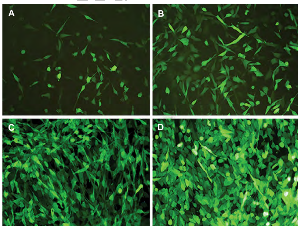
Fig.4: Antibiotic selection of transduced U-251 MG cell line. The stable cell line was produced by puromycin selection after 7 days. A, B. Depict the second and third day after using puromycin (2 \mu g/ml), C and D. Show the 5 th and 7 th day of selection.
