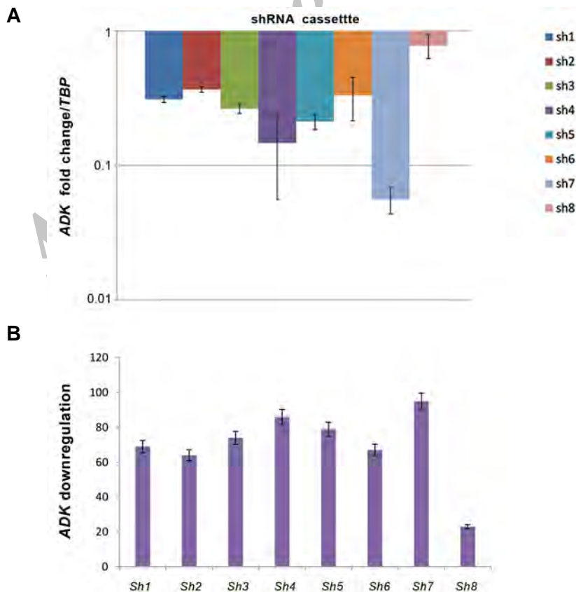
Fig. 5: Screening of anti-ADK miR-shRNAs in U-251 MG cells by semiquantitative real-time polymerase chain reaction. A. The expression of ADK mRNA was evaluated in the lentiviral-engineered U-251 MG cells by REST 2009 software. For improving the reliability of real-time polymerase chain reaction (RT-PCR), TBP was used as a reference gene and B. Percent of ADK knockdown obtained by anti-ADK miR-shRNAs. Data showed that anti-ADK miR-shRNAs (except for sh8) could knock down ADK more than 60% and sh4 and sh7 were the most efficient with 86 and 95% ADK knockdown, respectively.
