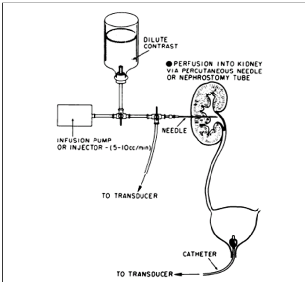
Figure 3. Whitaker test setup. Absolute pressure differences across the ureter are obtained by subtracting bladder pressure from renal pelvis pressure, which also cancels the effect of intra-abdominal pressure.
