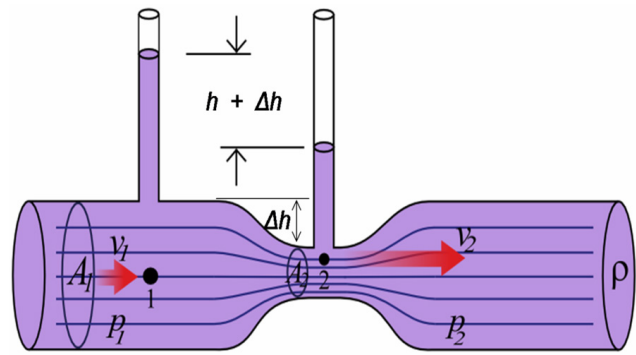
Figure 2. The pressure at "1" is higher than at "2" and the fluid speed at "1" is lower than at "2" because the cross-sectional area at "1" is greater than at "2".
