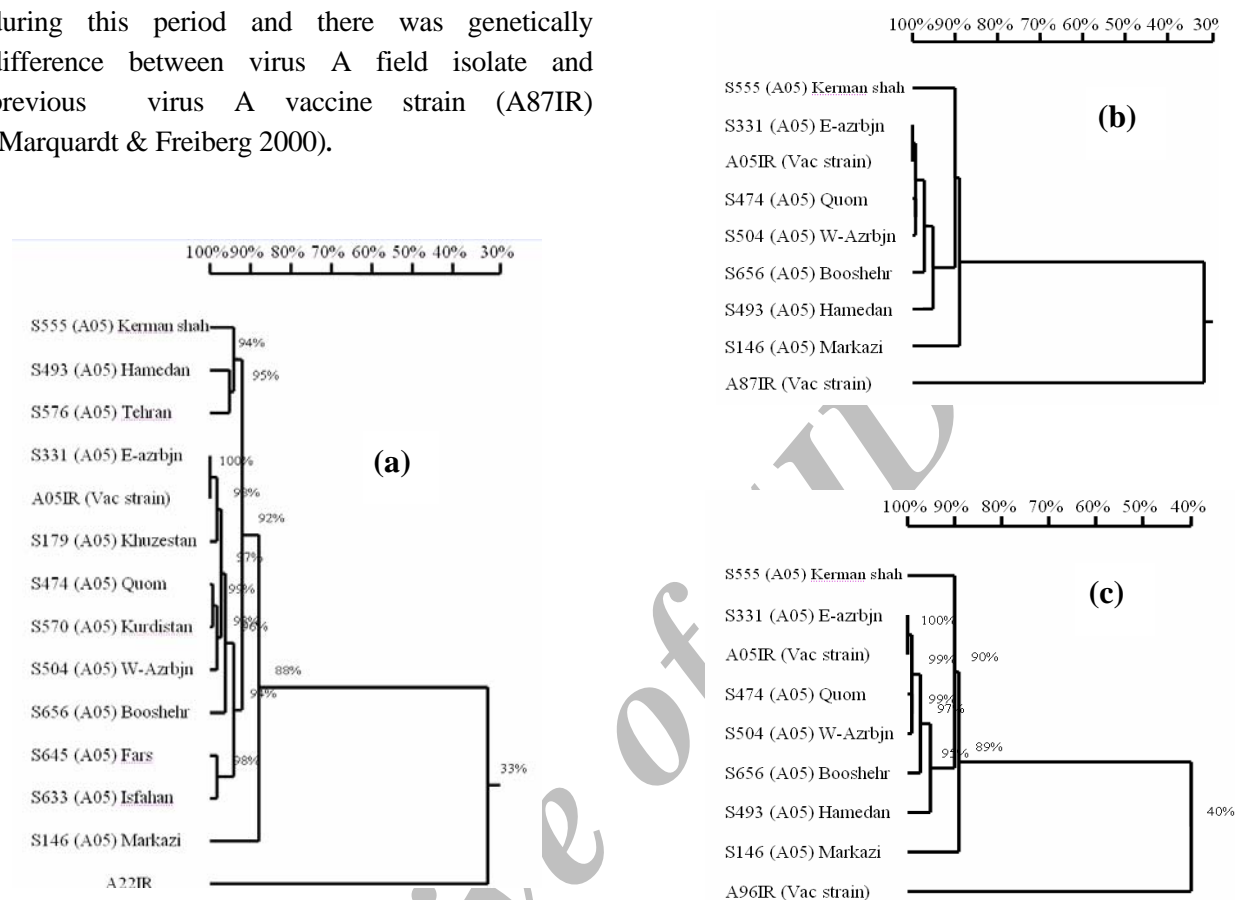
Figure 1. dendrogram based on alignment of 600 bp of the 3' end of the VP1 sequences of isolates Type A from the outbreaks in Iran during 2005–2006 compare with representative of type A 22 IR isolate identified previously and new vaccine strains A05(a), and A 87 Iranian vaccine strain (b) and A 96 vaccine strain (c).
