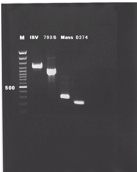
Figure 1. The typical results of molecular tests. The PCR products of 1200, 972, 295 and 217 bps length were amplified for detection of IBV, 793/B, D274 and Massachusetts types respectively.
