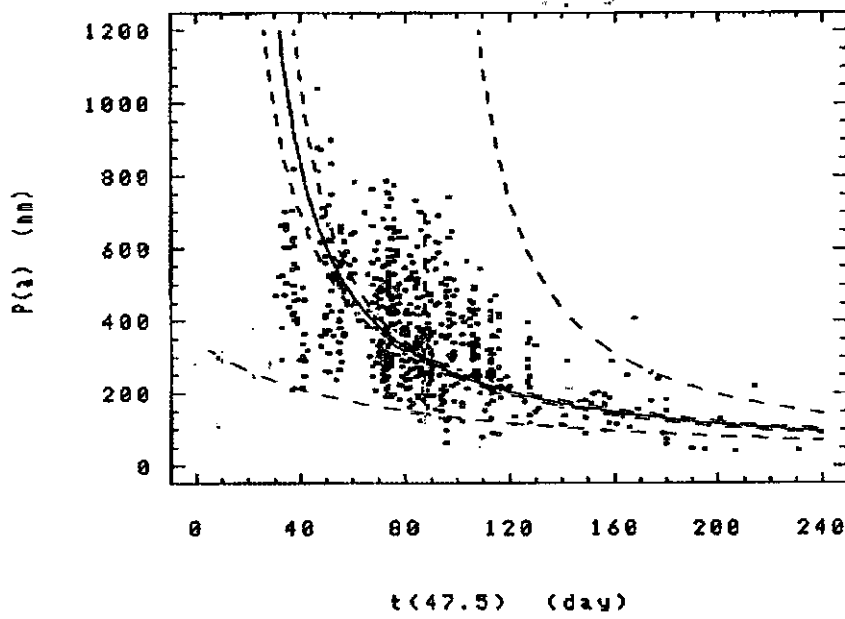
Fig.2. Reciprocal relationship between annual precipitation and t_{47.5} for the southern province.
