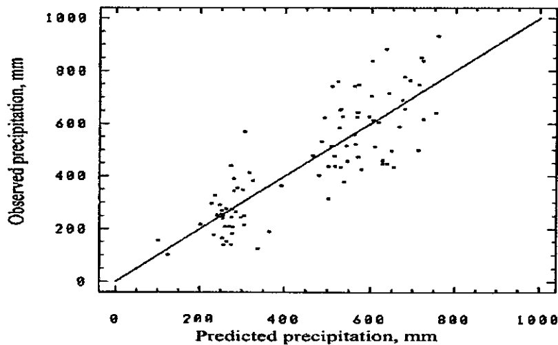
Fig.4. The relationship between observed and predicted annual precipitations for five stations in southern province.
