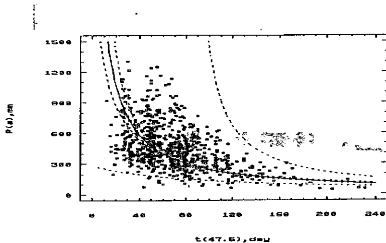
Fig.3. Reciprocal relationship between annual precipitation and t_{47.5} for the western province.
