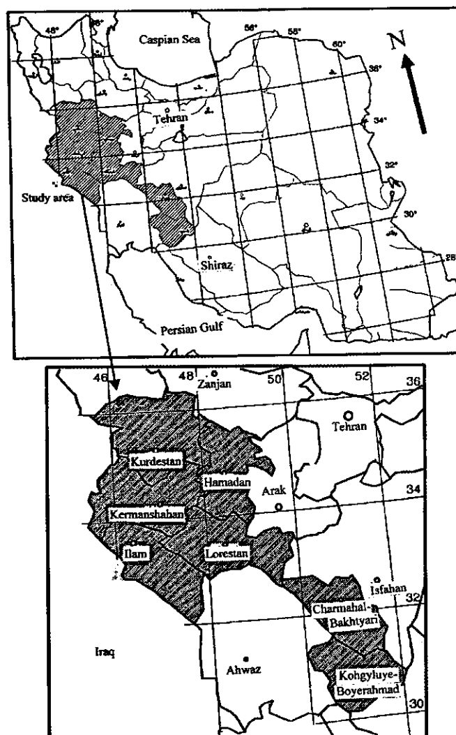
Fig.1. Location of the study areas.
