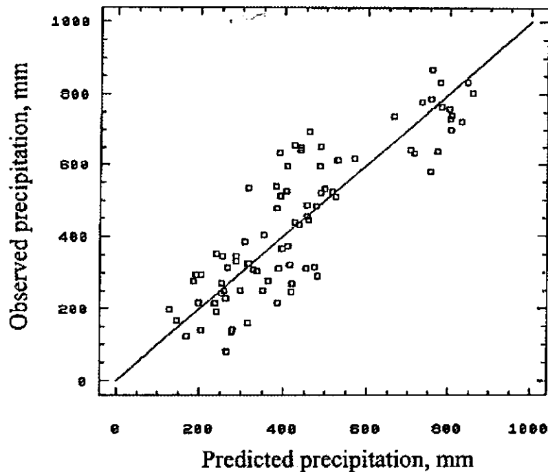
Fig.5. The relationship between observed and predicted annual precipitations for seven stations in western provinces.
