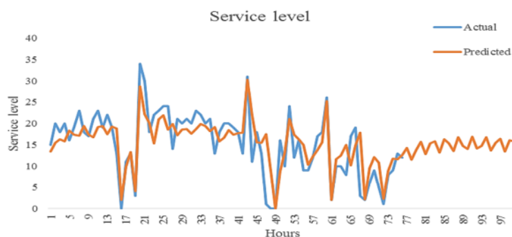
Fig. 9. Actual and predicted values of service level
