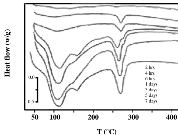
Fig. 2: DSC thermographs of the Secar 71 hydrated at 12 °C.
