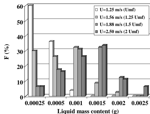
Fig. 3: Liquid mass content distribution of coated particles as a function of the fluidizing gas velocity U (liquid binder flow rate 2 \times 10^{-6} m 3 /s, gas jet flow rate 0.0015 m 3 /s).
