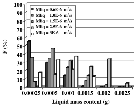
Fig. 7: Size distribution in different liquid binder flow rate, fluidizing gas flow rate 0.0092 m 3 /s, gas jet flow rate 0.0015 m 3 /s.
