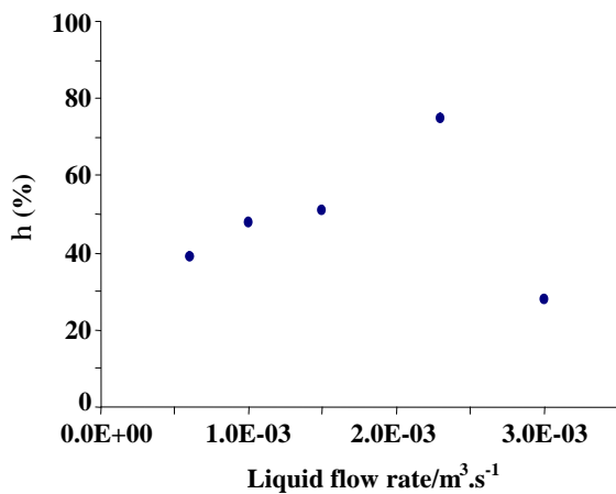
Fig. 8: Coating efficiency in different liquid binder flow rate, fluidizing gas flow rate 0.0092 m 3 /s, gas jet flow rate 0.0015 m 3 /s.
