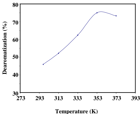
Fig. 5: Effect of temperature on dearomatization on SMZ.
