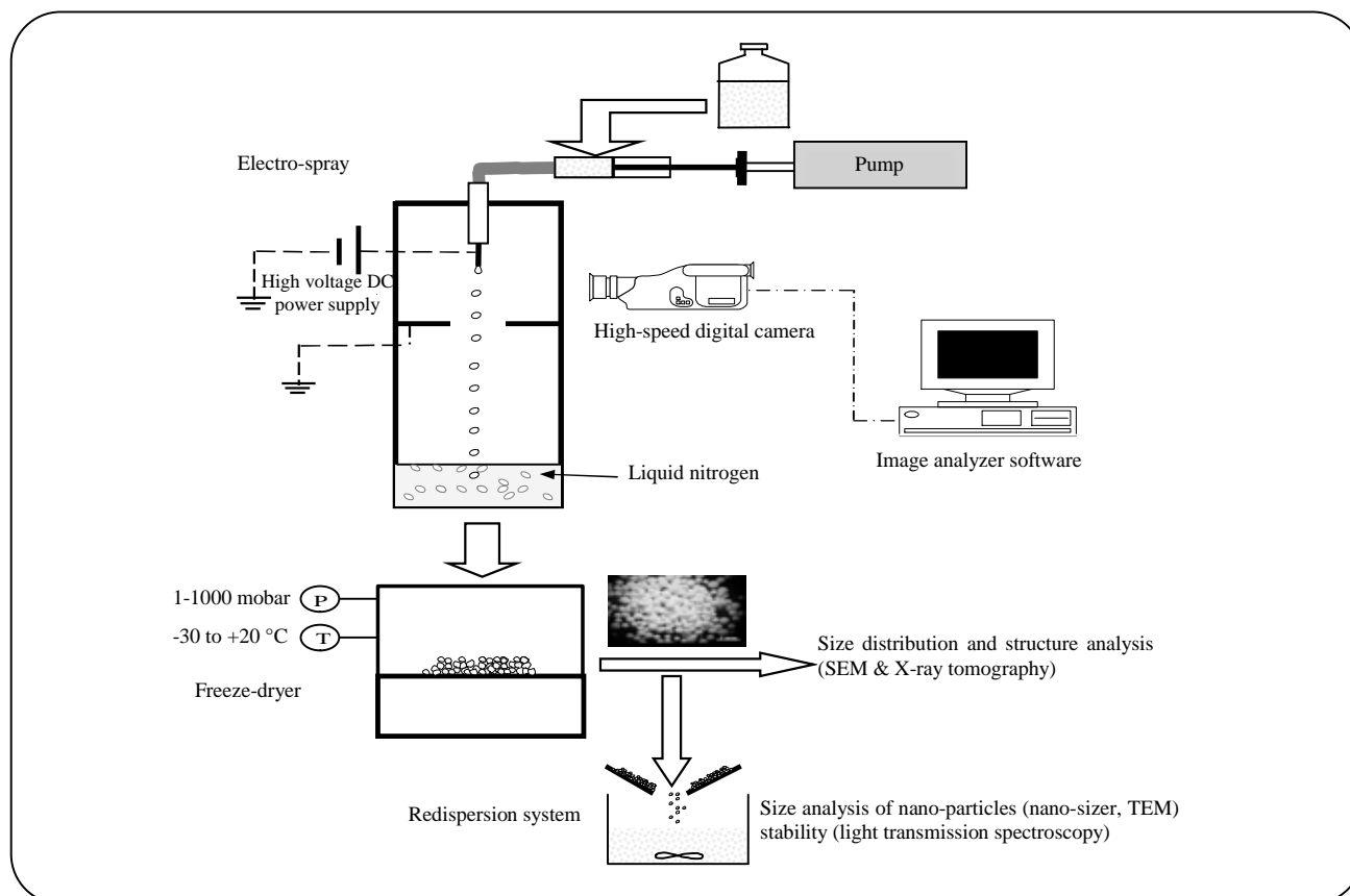
Fig. 2: Schematic drawing of combined process of electro-spraying and freeze-drying.
