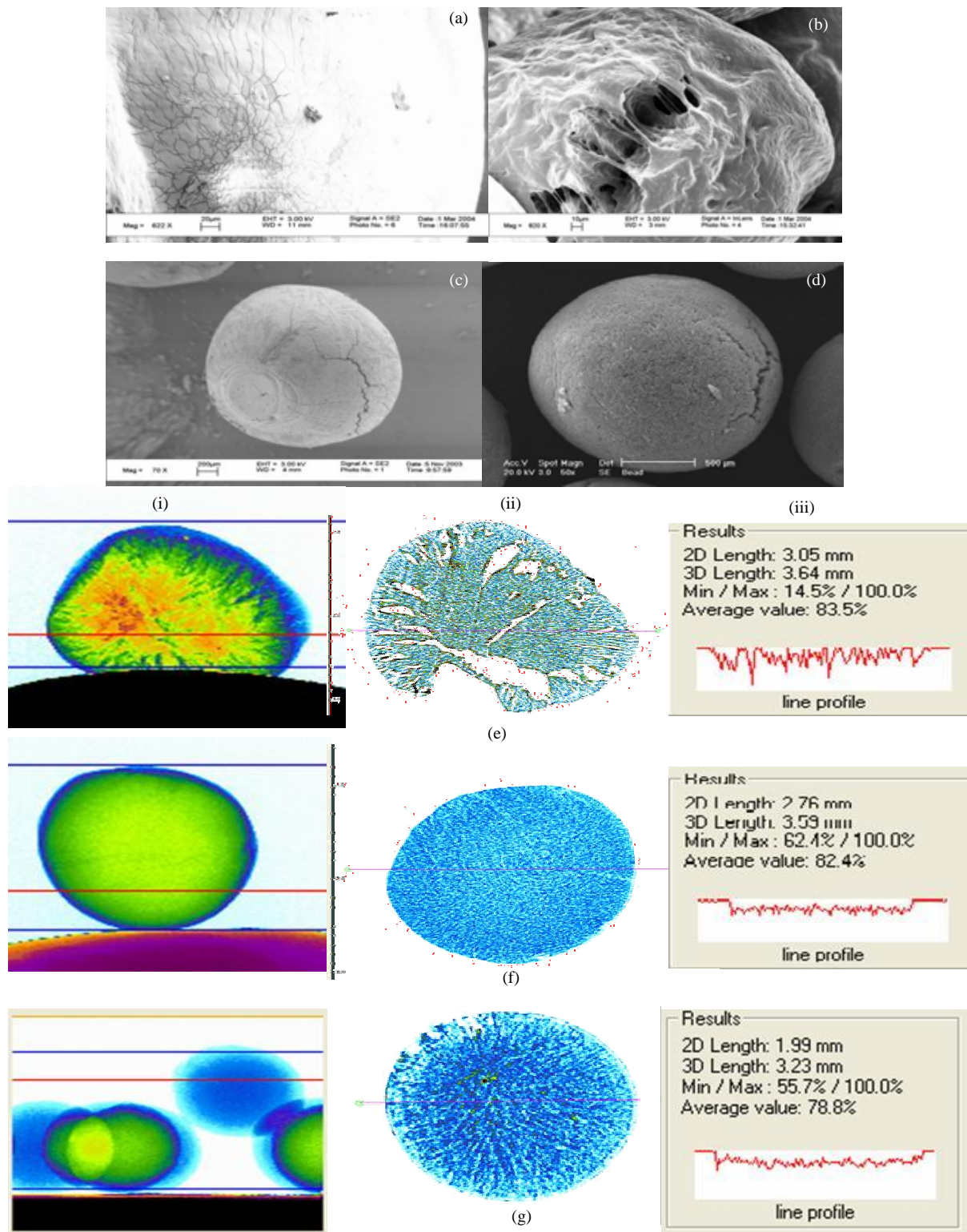
Fig. 5: SEM and X-ray tomography images of nanoparticle assemblies produced by freeze drying at different voltages. SEM images are: a) latex, 0 kV; b) latex, 8 kV; c) silica, 0 kV; d) titania with 7 % PEG, 4 kV; and X-ray tomography images are: e) latex 0 kV; f) silica 0 kV; and g) titania 4 kV.
