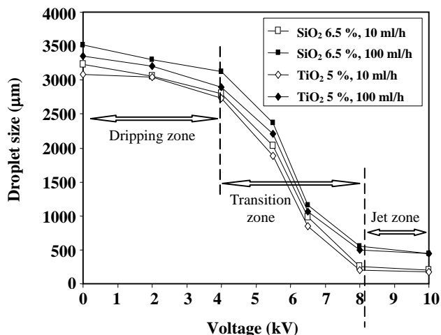
Fig. 4: Effect of DC voltage on droplet size of silica and titania at two different flow rates.
