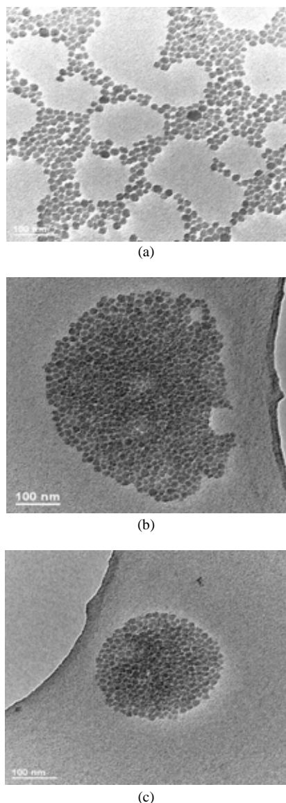
Fig. 8: TEM images of colloidal silica solutions a) initial stabilised system b) and c) partially dispersed showing integrated clusters.
