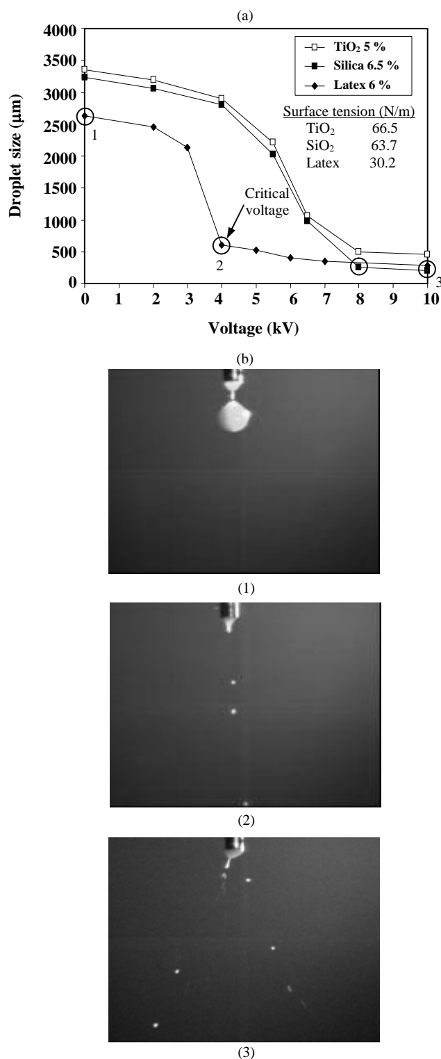
Fig. 3: Effect of DC electric field on size of droplets and pattern of spraying (a) graphs of droplet size versus voltage (b) images of spraying droplets at different conditions acquired by high-speed digital recordings of 1) no voltage, 2) 4 kV, and 3) 10 kV.
