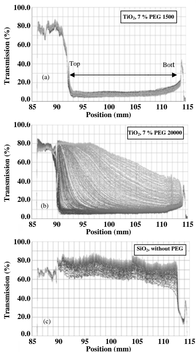
Fig. 7: Stability analysis results of redispersion of titania (containing 7 % PEG 1500 and 20000) and silica without PEG using a centrifugal light transmission apparatus under the same operating conditions.
