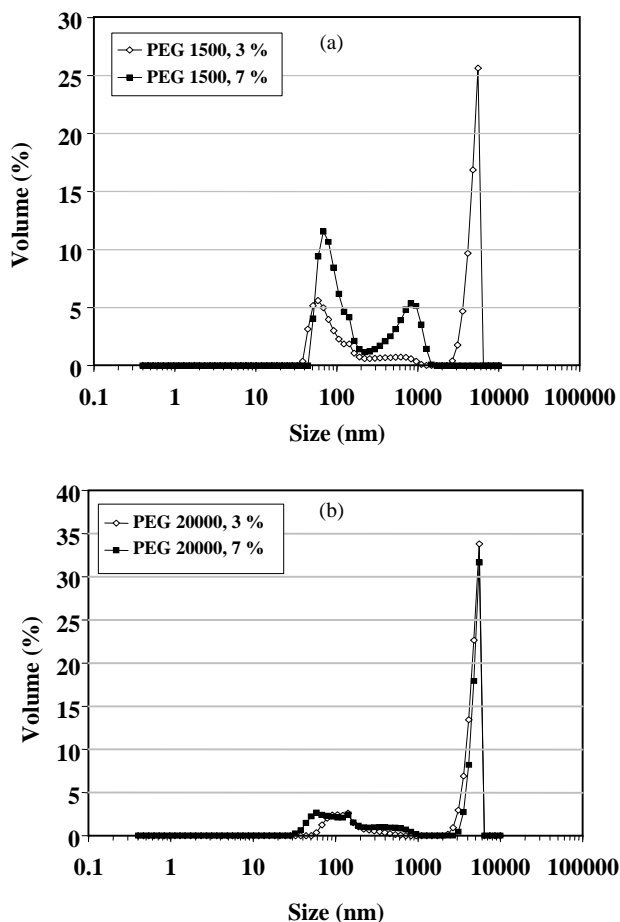
Fig. 9: Size distribution of redispersed \text{TiO}_2 nanoparticle assemblies containing different molecular weights and concentrations of PEG a) Mw 1500, b) Mw 20000.
