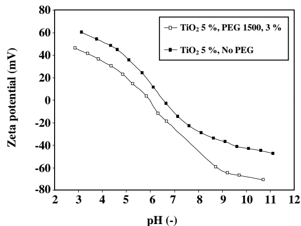
Fig. 1: Effect of pH on interparticle potential of solutions made with and without PEG shown as zeta potential vs pH.
