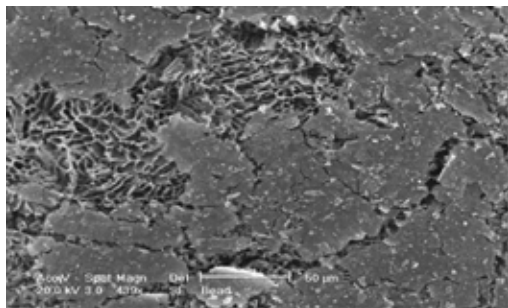
Fig. 6: SEM image of surface of a freeze-dried \text{TiO}_2 nanoparticle assembly using initial colloidal solution of 5 % \text{TiO}_2 and 7 % PEG 1500.
