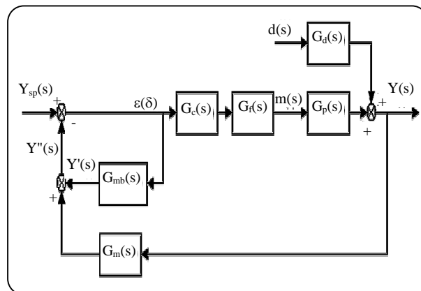
Fig. 6: Block diagram of a MBPL-predictor time-delay compensating loop with the capability to remove offset with a PI controller.
