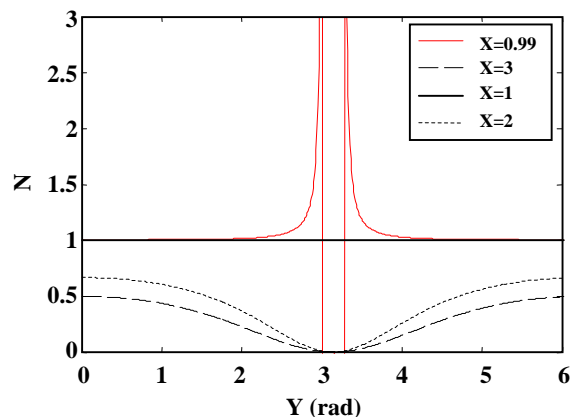
Fig. A - 2: Variations of z = (1 + \cos(\beta - \alpha)) / (|A|/|B| + \cos(\beta - \alpha)) with Y = (\beta - \alpha) and X = |A|/|B| .
