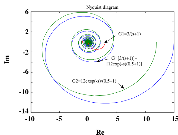
Fig. 5: The Nyquist plot of G(j\omega) = G_1(j\omega) + G_2(j\omega) traces the Nyquist plot of G_2(j\omega) in a resonating behavior, where |G_1(j\omega)| < |G_2(j\omega)| ; \forall \omega . G(j\omega) = (3/s+1) + 12e^{-s}/(0.5s+1) .
