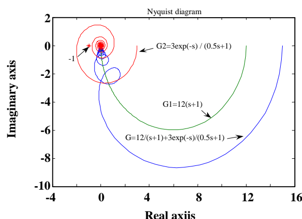
Fig. 4: The Nyquist plot of G(j\omega) = G_1(j\omega) + G_2(j\omega) traces the Nyquist plot of G_1(j\omega) in a resonating behavior, where |G_1(j\omega)| > |G_2(j\omega)| ; \forall \omega .
