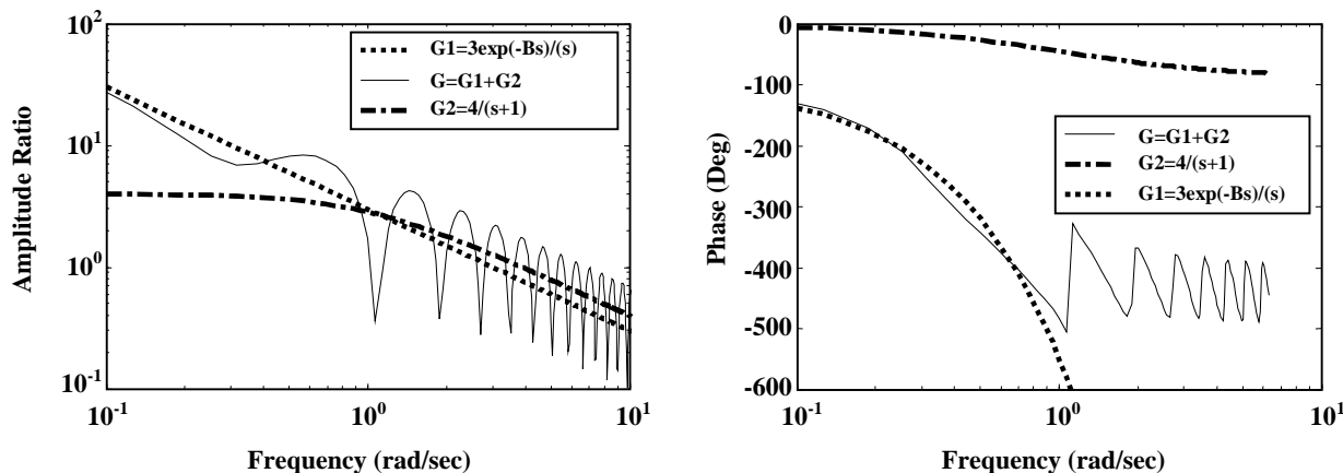
Fig. 8: A crossing of gains of the predictor, G_{mb}(s)=4/(s+1) , and the simple-open-loop-transfer-function, 3e^{-8s}/s , appear at lower frequencies when using PI controller.
