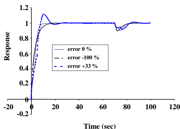
Fig. 10: Controlling the Ir-TF systems by MBPL-predictor.
