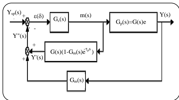
Fig. 1: Smith predictor control loop.
