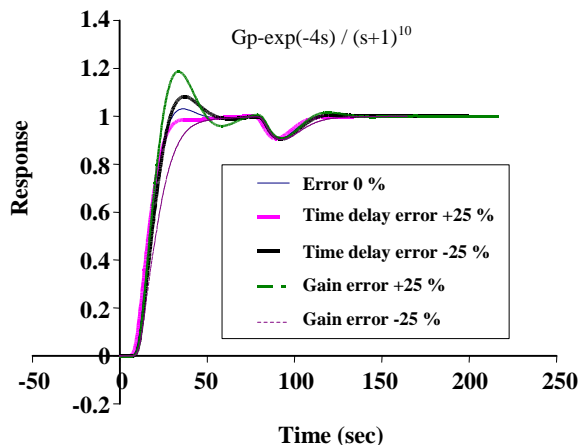
Fig. 12: Controlling high order models by MBPL-predictor.
