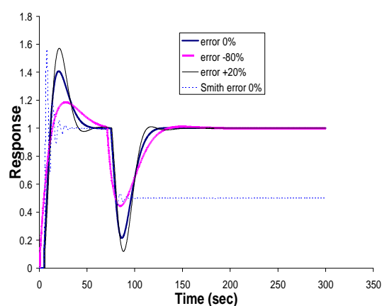
Fig. 11: Response of the MBPL-predictor to step input in set point and load input for an integrator system with time-delay.
