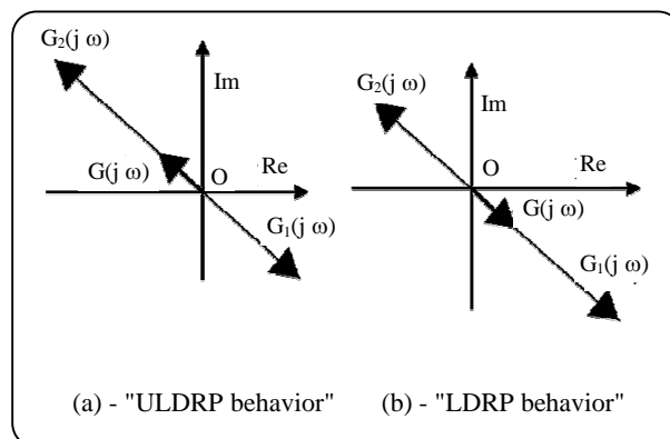
Fig. 3: Detecting the origin of appearance of dual phase behaviors in frequency response of Ir-TF models.
