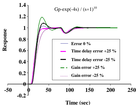
Fig. 12: Controlling high order models by MBPL-predictor.
