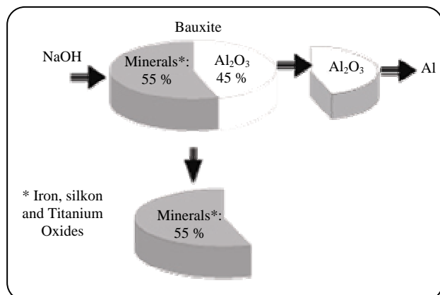
Fig. 1: Aluminium oxide is dissolved out of the bauxite and processed further to aluminium. The residue containing a mixture of naturally occurring minerals is then transferred to a disposal site.
