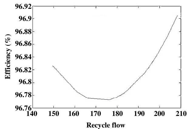
Fig. 3: Effect of recycle flow rate on efficiency at Constant jet-impingement and feed flow rates, Feed flow rate=358.0 m 3 /h, Jet flow rate=76.9 m 3 /h.
