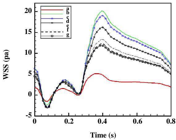
Fig. 12: WSS curves on the points a, b, c, d, e, f and g in the ac-7530 bypass.
