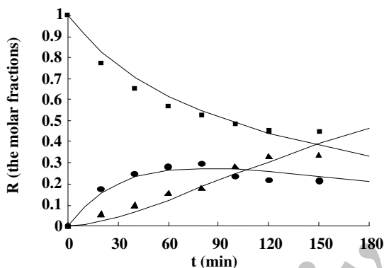
Fig. 5: Experimental data and model simulation of the molar fractions of L-Theanine in the feed ( R_f , ■), membrane ( R_m , ●) and receiving phase ( R_r , ▲) at 303.15 K.
