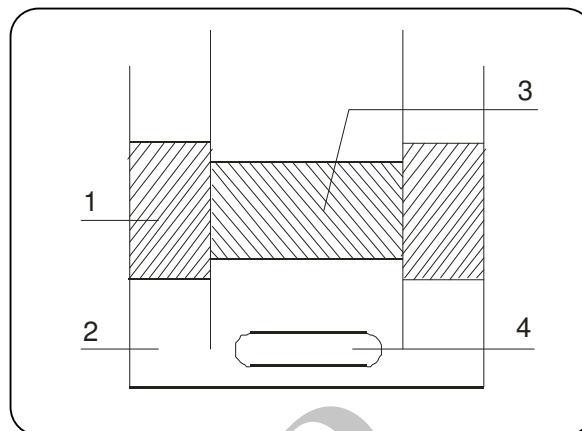
Fig. 1: Bulk liquid membrane separation vessel. 1. Receiving phase; 2. Organic membrane phase containing carrier; 3. Source phase; 4. Stirring bar.
