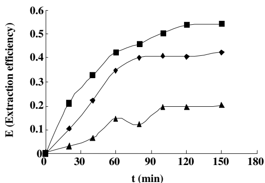
Fig. 2: Effect of initial concentration of L-Theanine on extraction efficiency. ■: initial concentration of L-Theanine is 1.8 g/L; ◆: 2 g/L; ▲: 1.4 g/L.
