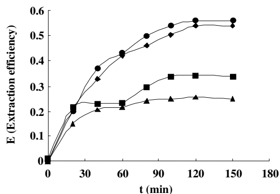
Fig. 3: Effect of carrier concentration in the membrane phase on extraction efficiency. ■: carrier concentration of 0.35 M; ▲: 0.25 M; ◆: 0.5 M; ●: 0.65 M
