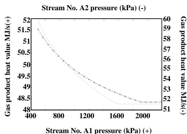
Fig. 8: Variation of the gas product heat value ( \text{MJ/s} ) against streams No. A1 & A2 pressure.
