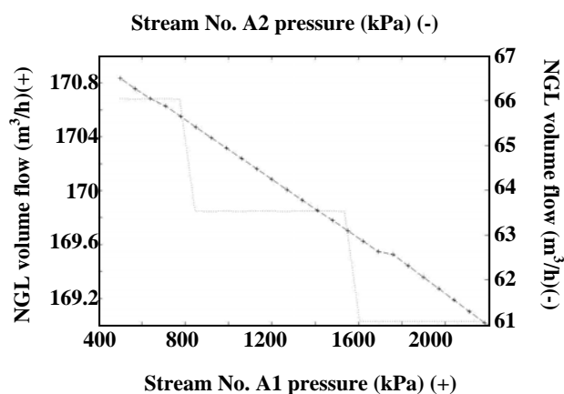
Fig. 6: NGL volume flow ( \text{m}^3/\text{hr} ) versus streams No. A1 & A2 pressures.
