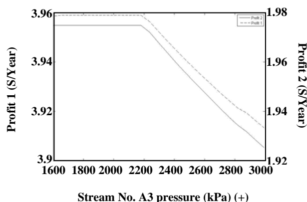
Fig. 14: The plant wide net profit against the stream No.A3 pressure.
