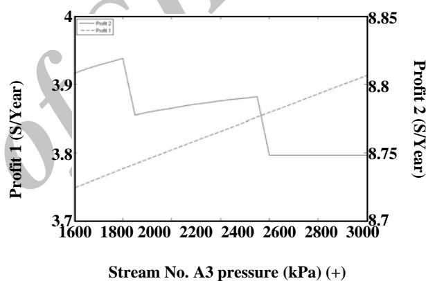
Fig. 15: The plant wide net profit against column operating pressure.
