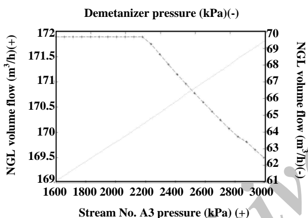
Fig. 7: NGL volume flow ( \text{m}^3/\text{hr} ) versus stream No. A3 pressure and the column operating pressure.
