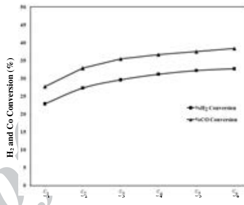
Fig. 5: Percentage H 2 and CO conversion variations with cobalt loadings.
