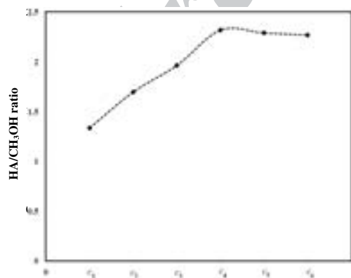
Fig. 8: Variations of HA/CH 3 OH ratio with %Mo loadings.
