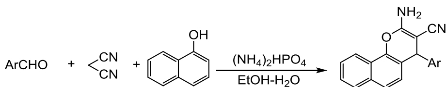
Scheme 1: Synthesis of 2-amino-4H-chromenes catalyzed by diammonium hydrogen phosphate.
