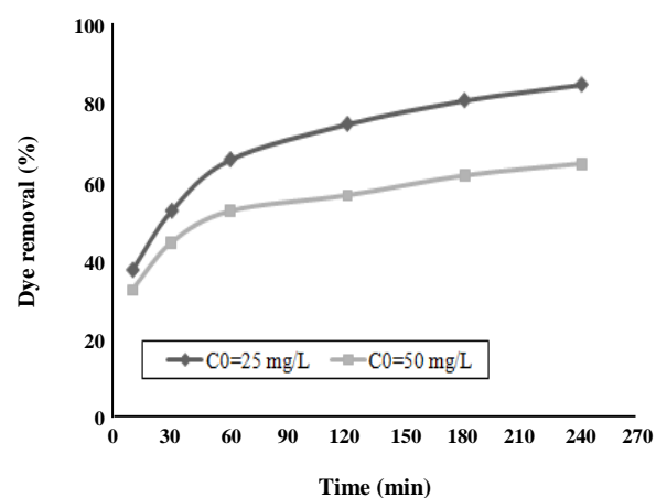
Fig. 4: Effect of contact time on the adsorption capacity of RR198 dye.
