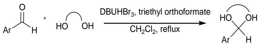
Scheme 3: Acetalization of aromatic aldehydes with diols in the presence of DBUH-Br3.
