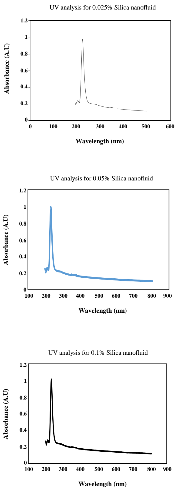
Fig. 1: Analysis of Nanofluid using UV Spectroscopy.
