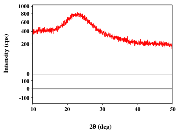
Fig. 2: Characterization of silica nanofluids using XRD analysis.
