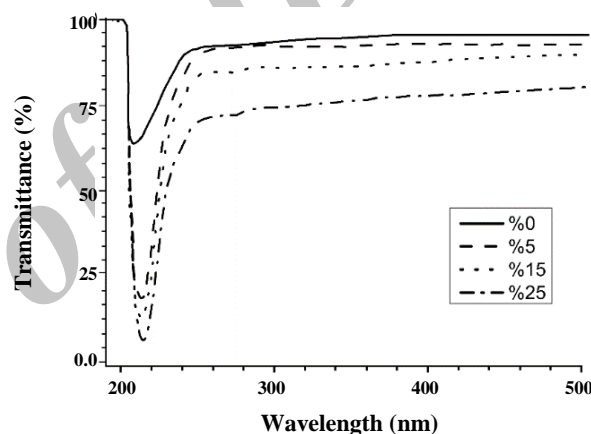
Fig. 4: UV-vis transmittance spectra of \text{SnO}_2 nanoparticles for Al-doped.
