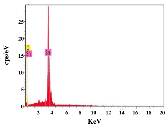
Fig. 9: EDX analysis of SnO 2 nanoparticle.
