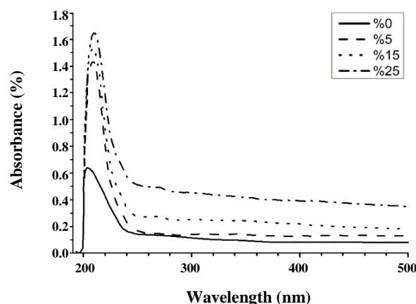
Fig. 5: UV-vis absorbance spectra of \text{SnO}_2 nanoparticles for Al-doped.
