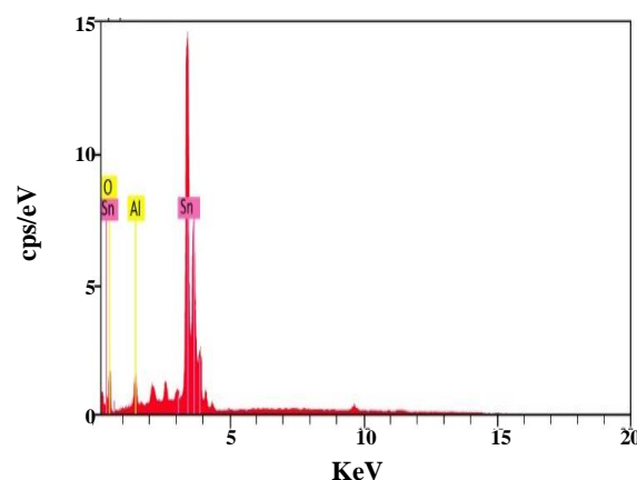
Fig. 10: EDX Analysis of SnO 2 Nanoparticle with Al-doped (25%).
