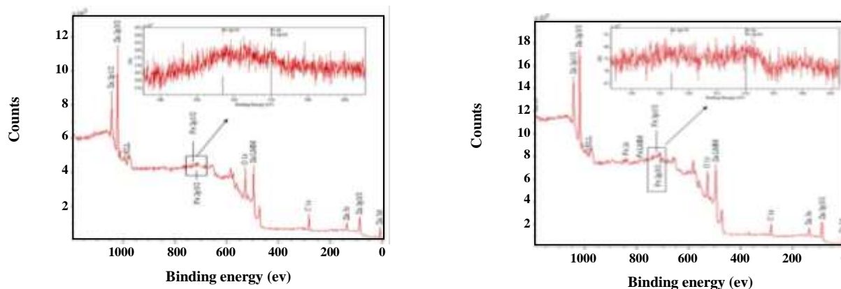
Fig. 5: XPS spectra of Zn_{1-x}Fe_xO for (a) x=0.05\% and (b) x=0.07\% .
