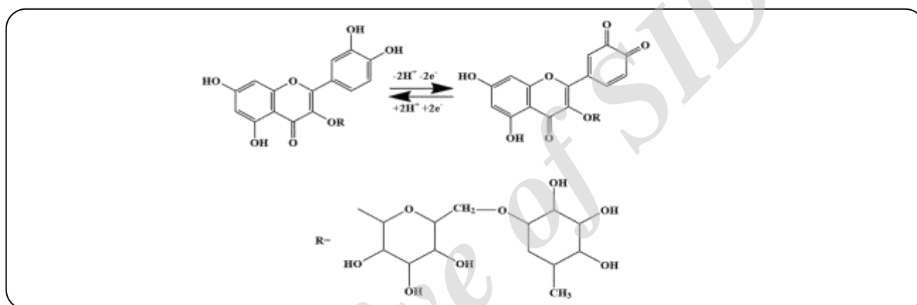
Scheme 1. A proposed redox mechanism of rutin on the SIL-GO/GCE.
