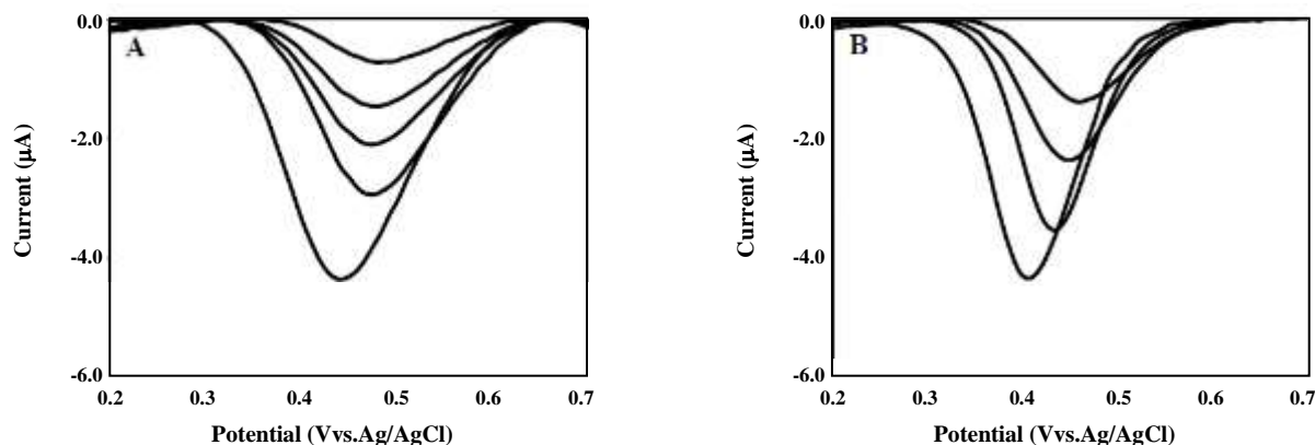
Fig. 5: (A) Differential pulse voltammograms of 5\mu\text{M} quercetin at SIL-GO/GCE in 0.1\text{ M} phosphate buffer solution (pH 7.0) in the present and absent of different dsDNA concentrations. dsDNA concentrations (from top to bottom): 0.0 , 1.0 , 2.0 , 3.0 , and 5.0\ \mu\text{M} . (B) Differential pulse voltammograms of 5\mu\text{M} hesperidin at SIL-GO/GCE in 0.1\text{ M} phosphate buffer solution (pH 7.0) in the present and absent of different dsDNA concentrations. dsDNA concentrations (from top to bottom): 0.0 , 1.0 , 3.0 , and 5.0\ \mu\text{M} .
